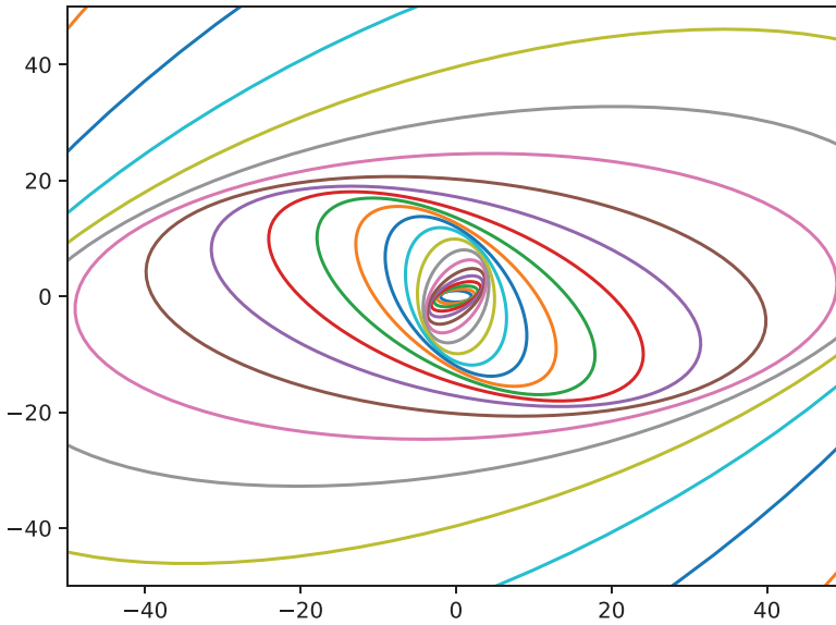
FIGURE 2 The convex foliation (\mathcal{E}(t))_{t \in \mathbb{R}} for a(t) = 2b(t) = 2e^t
