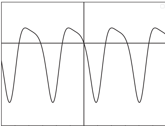
FIGURE 4 Plot of h(\theta) = \frac{\sqrt{2}}{1+\cos^2 \theta} - \frac{1+\sin^2 \theta}{\sqrt{2}-\cos \theta \sin \theta}
