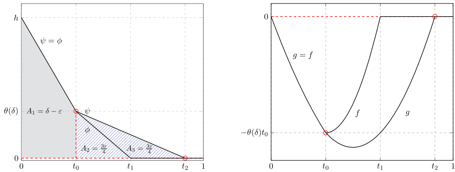
Fig. 2 Left: Regions below the functions \psi and \phi . Right: The functions g(t) = -t\psi(t) and f(t) = -t\phi(t) coincide on [0, t_0] while for t \geq t_0 we have f \geq g
