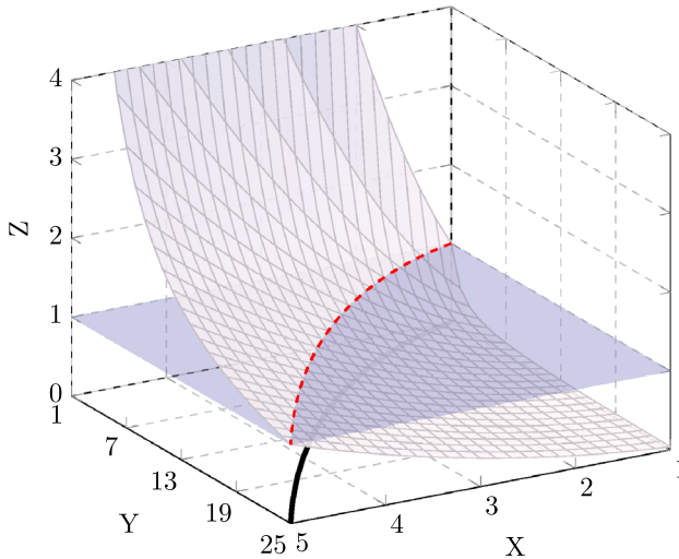
Fig. 1 Function g(x, y) = x^2/y . In blue, the plane z = 1 . In black, the curve \gamma(t) for c = 1 . In dashed red, the curve (\gamma(t), g(\gamma(t))) = (\gamma(t), c) for c = 1 . Plane XY plotted in 1:6, starting at point (1,1). Plane XZ plotted in 1:1, starting at point (1,0)
